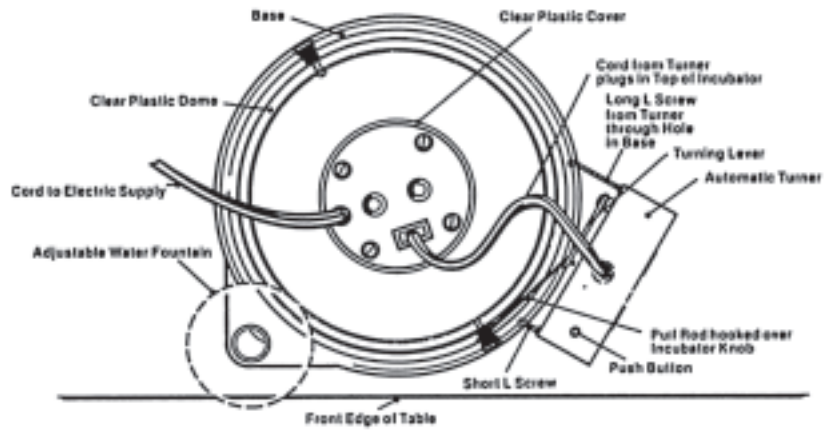
TOP VIEW OF INCUBATOR WITH AUTOMATIC TURNER
